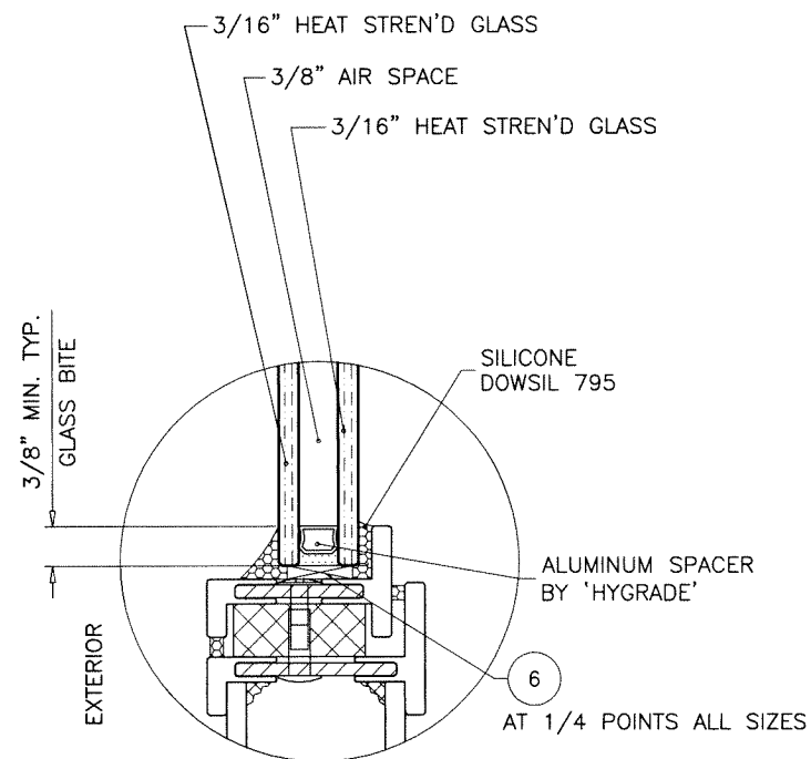
GLAZING DETAIL 3/4" OVERALL INSUL. GLASS
